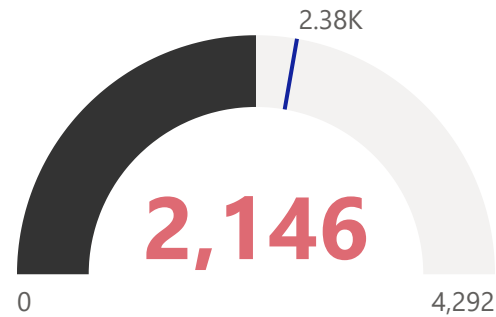
Monthly Orders vs Target
